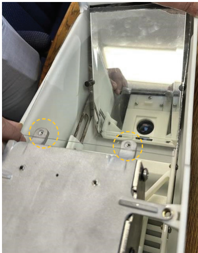
23.21 Aligning the Holes
